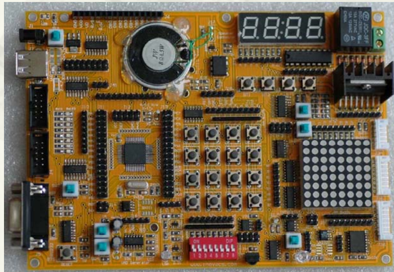
1. AVR Experiment Board
