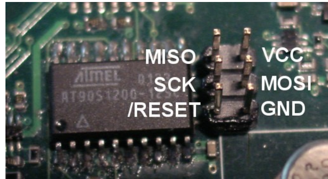
Figure 5 - ISP Pinout
