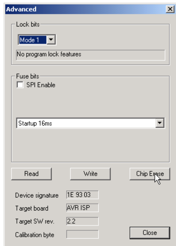
Figure 6 - Advanced Programming Options
