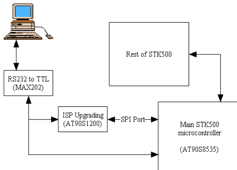
Figure 1 - STK500 command interface diagram
