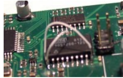
Figure 3 - Connecting all the reset pins to GND
